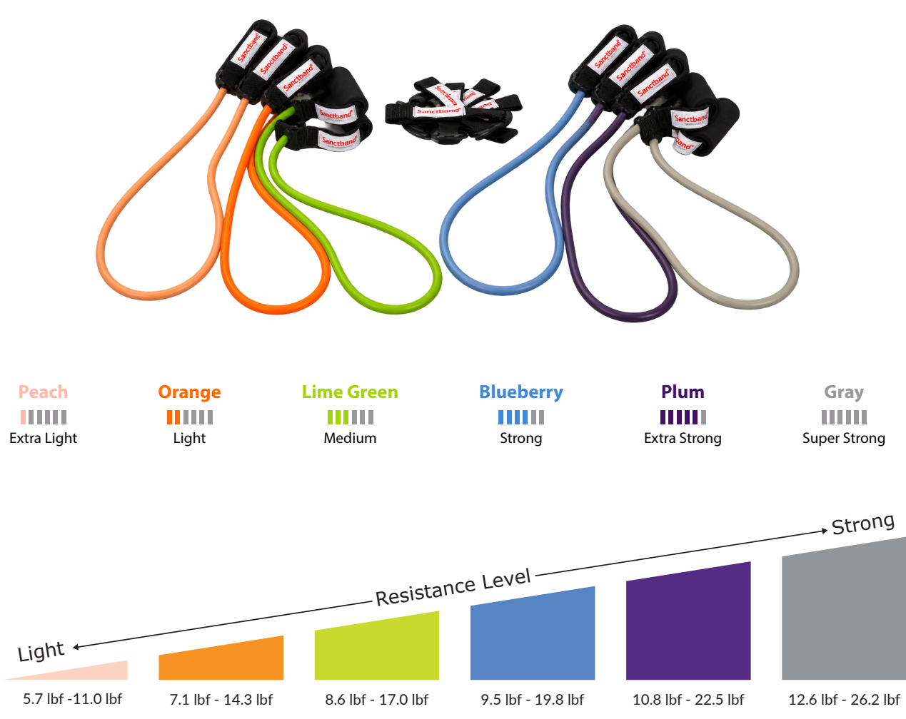
Typical Pull Force Chart With An Elongation Percentage of 100% to 300%
